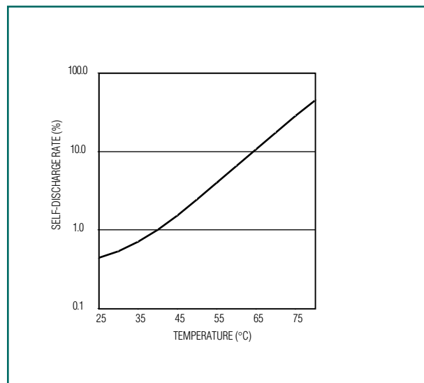
Figure 4. The self-discharge rate increases as temperature increases.
